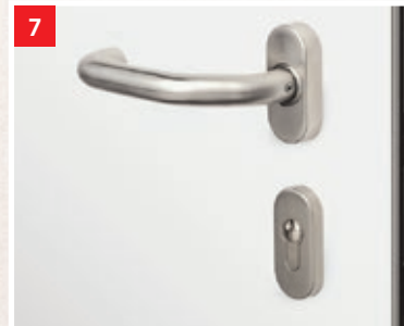
Stainless steel handle ART. 6039 with cylinder rosette ART. 6007 inside
